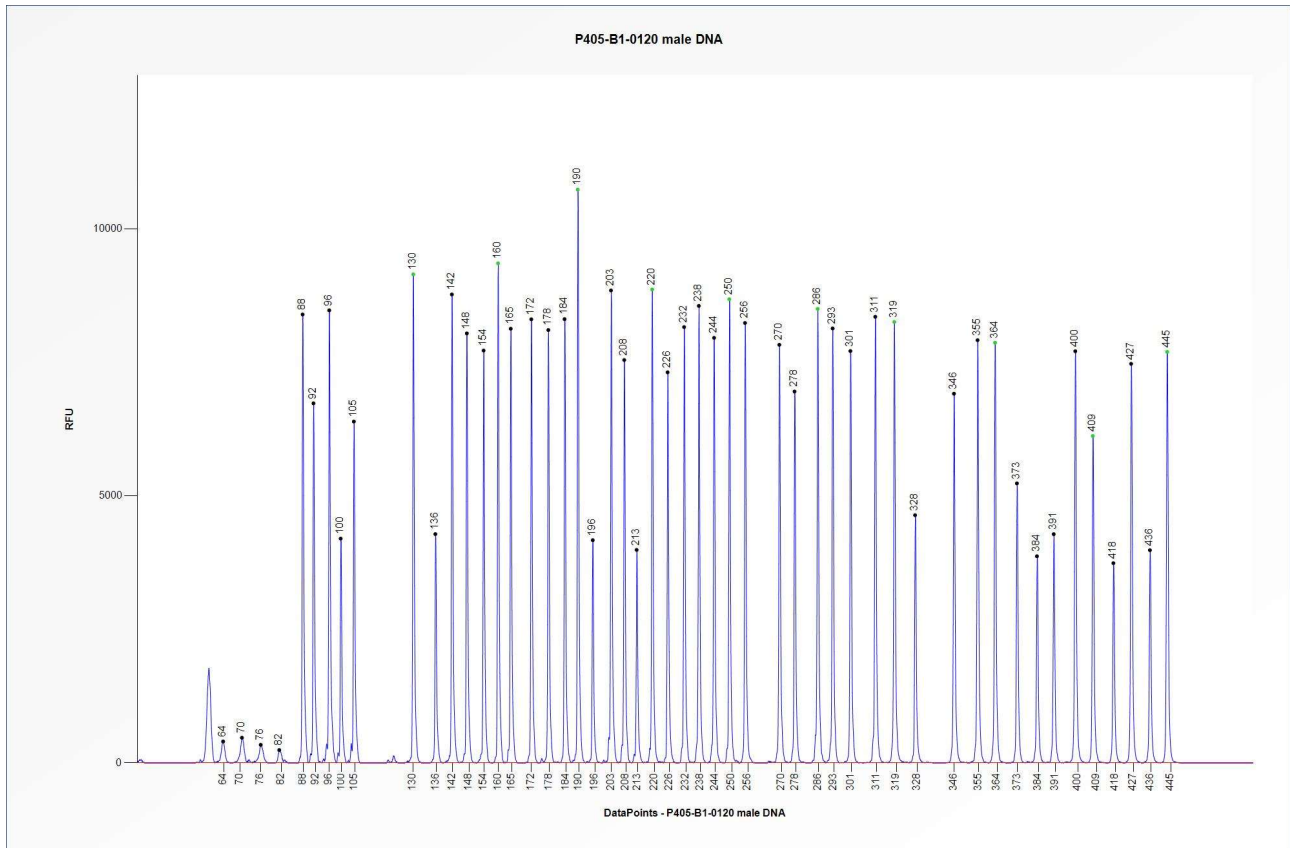
Figure 1. Capillary electrophoresis pattern from a sample of approximately 50 ng human male control DNA analysed with SALSA MLPA Probemix P405 CMT1 (B1-0120).
