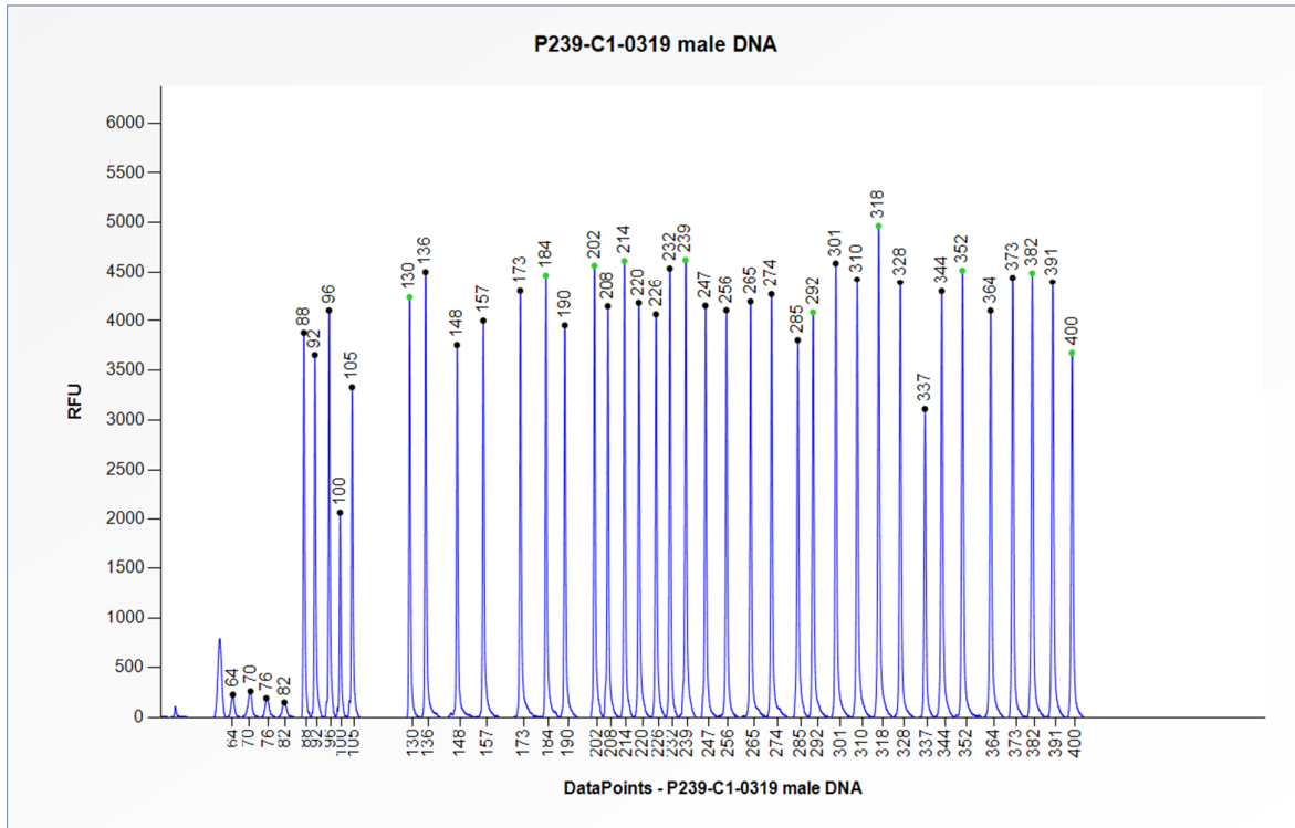
Figure 1. Capillary electrophoresis pattern from a sample of approximately 50 ng human male control DNA analysed with SALSA MLPA Probemix P239 BRCA1 region (C1-0319).
