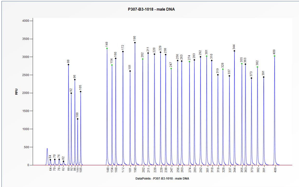
Figure 1. Capillary electrophoresis pattern from a sample of approximately 50 ng human male control DNA analysed with SALSA MLPA Probemix P307 SEPT9 (B3-1018).
