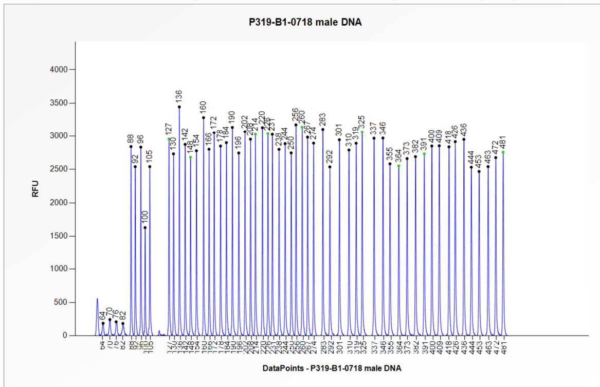
Figure 1. Capillary electrophoresis pattern from a sample of approximately 50 ng human male control DNA analysed with SALSA MLPA probemix P319 Thyroid (B1-0718).
