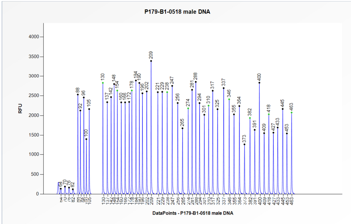
Figure 1. Capillary electrophoresis pattern from a sample of approximately 50 ng human male control DNA analysed with SALSA MLPA probemix P179 Limb malformations-1 (B1-0518).
