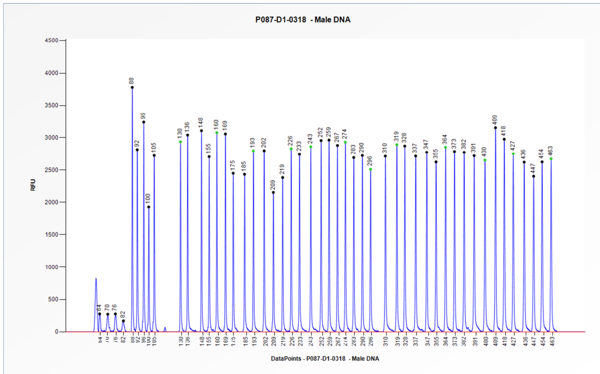
Figure 1. Capillary electrophoresis pattern from a sample of approximately 50 ng human male control DNA analysed with SALSA MLPA probemix P087 BRCA1 Confirmation (D1-0318).
