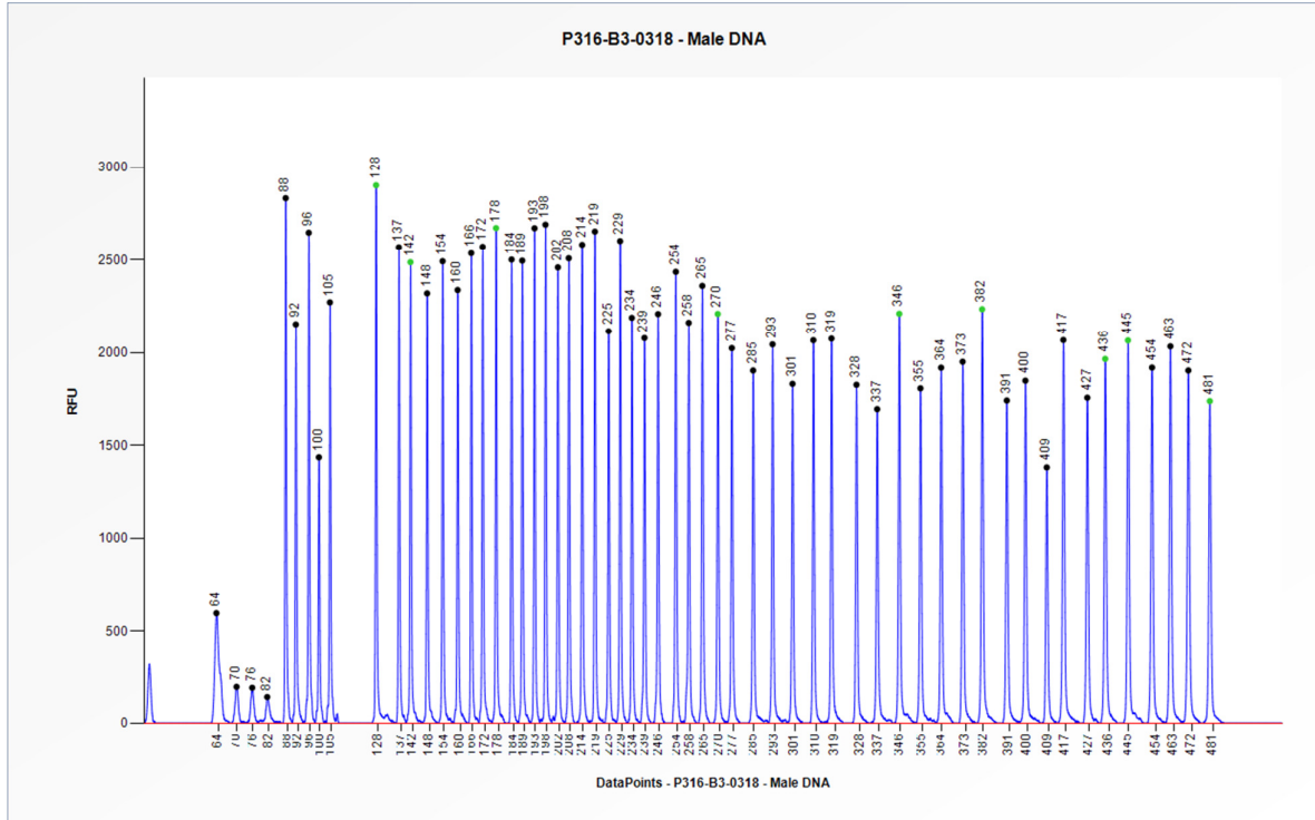
Figure 1. Capillary electrophoresis pattern from a sample of approximately 50 ng human male control DNA analysed with SALSA MLPA probemix P316 Recessive Ataxias (B3-0318).
