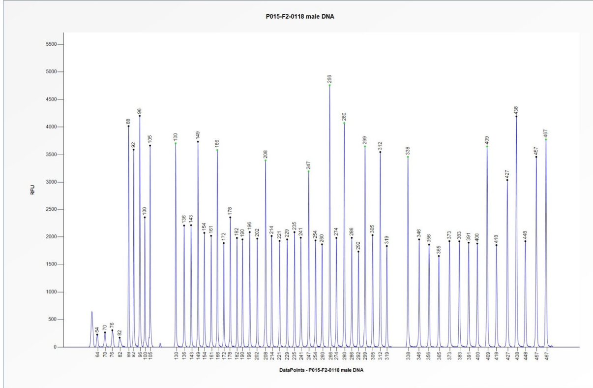
Figure 1. Capillary electrophoresis pattern from a sample of approximately 50 ng human male control DNA analysed with SALSA MLPA probemix P015 MEC2 (F2-0118).
